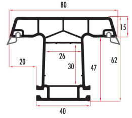
PEG62431 62 MM 4 ODACIKLI ORTA KAVIT / MULLION PROFILE PEG62432 (RENKLİ/COLORED)
